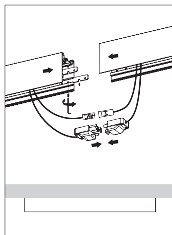
Lijnmontage Doorvoerbedrading 3x1.5mm 2 / 5x1.5mm 2 DALI Skyline 1200mm: max. 40 Skyline 1200mm Up/Down: max. 30 Skyline 1500mm: max. 30 Skyline 1500mm Up/Down: max. 25
